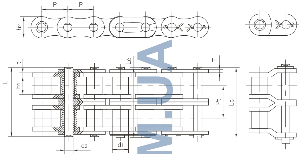
双排滚子链 Duplex roller chains
